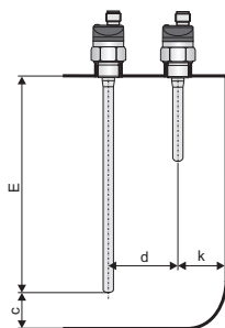
Fig. 1: Vertical mounting
