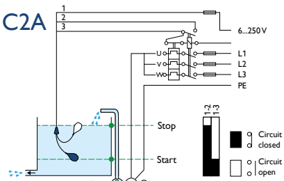
CHARGING-PUMP CONTROL
