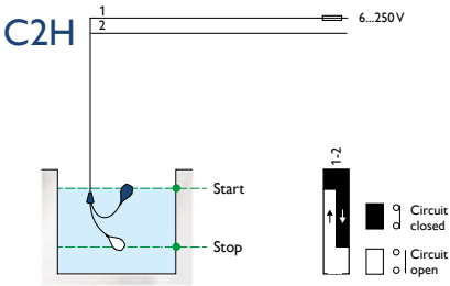
DISCHARGING-PUMP CONTROL
