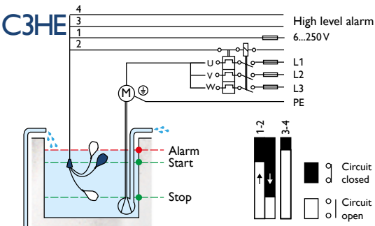
DISCHARGING-PUMP CONTROL + ISOLATED HIGH LEVEL ALARM
