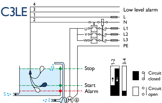
CHARGING-PUMP CONTROL + ISOLATED LOW LEVEL ALARM
