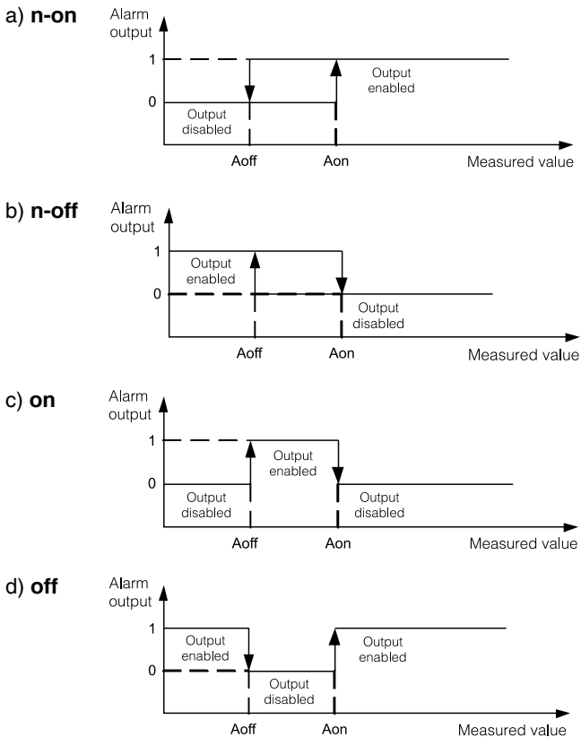
Fig. 8. Alarm types: a) n-on, b) n-off, c) on, d) off
