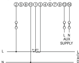
SINGLE PHASE 2-WIRE DIGITAL METERING SYSTEM (WITH EXTERNAL AUX.)
