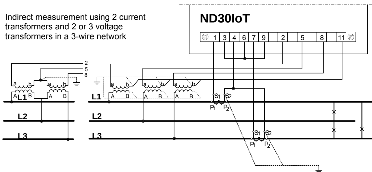
Fig. 7. Meter connections of input signals in a 3-phase 3-wire network
