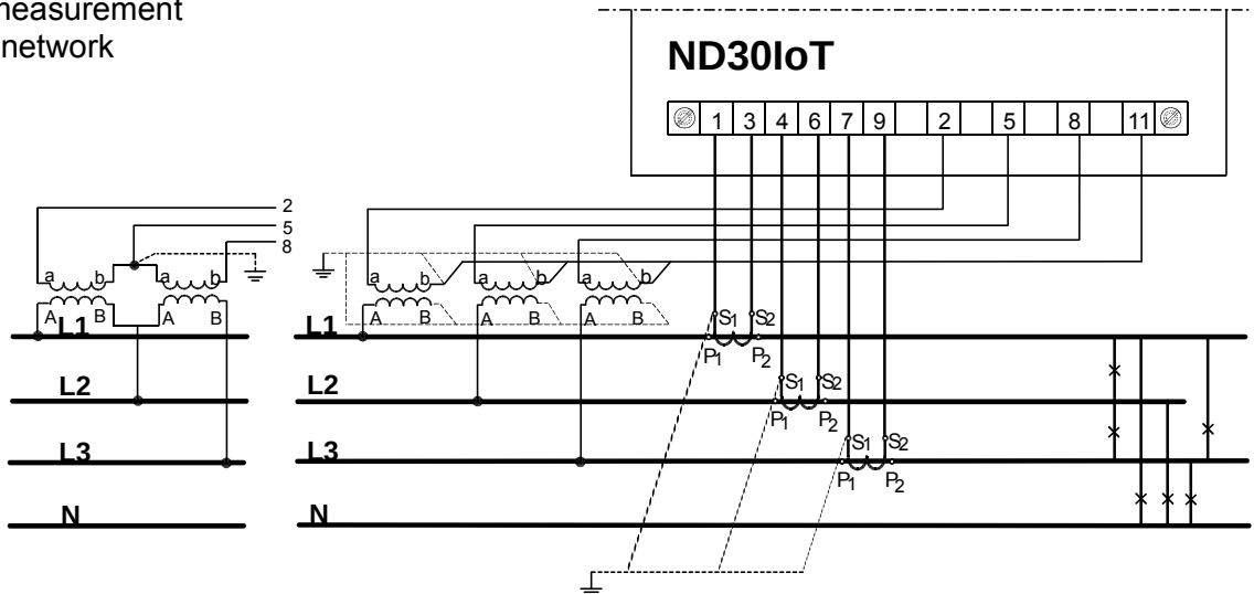
Fig. 6. Meter connections of input signals in a 3-phase 4-wire network
