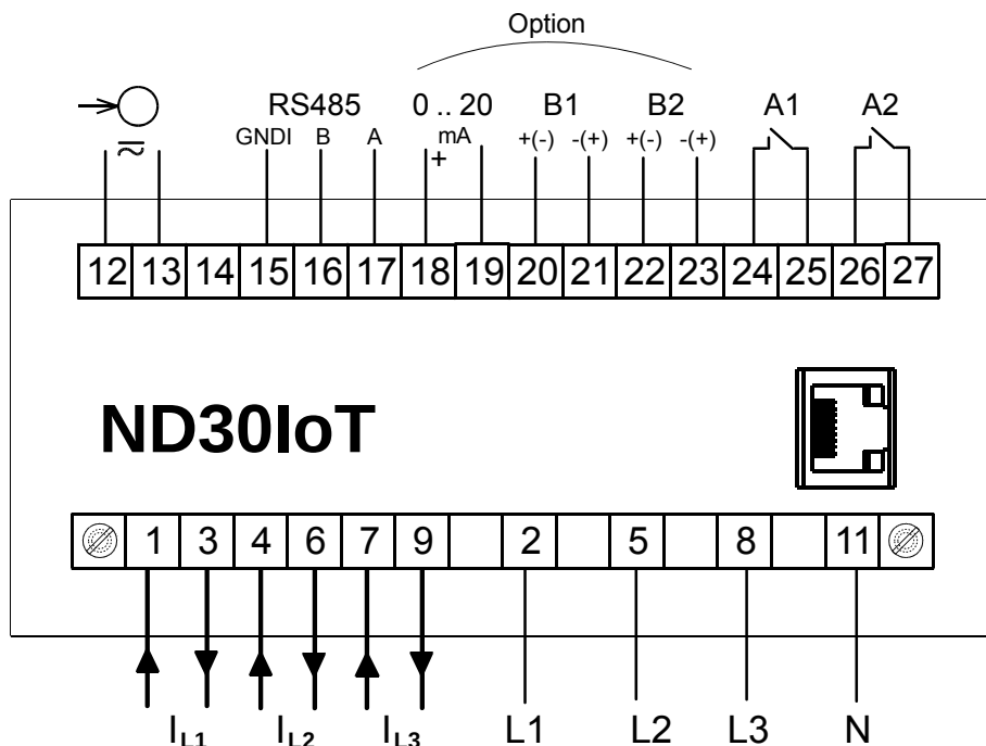
Fig. 4. Meter connections
