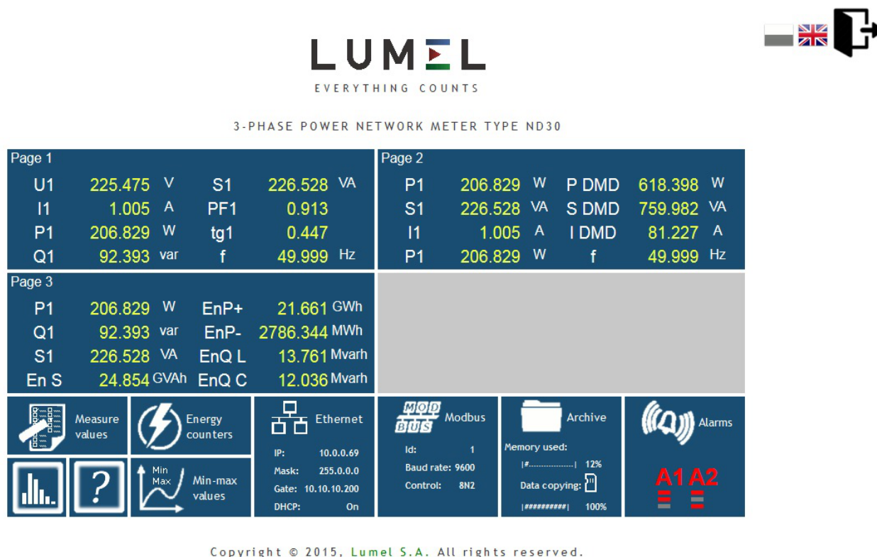
Fig. 29. View of the meter website
