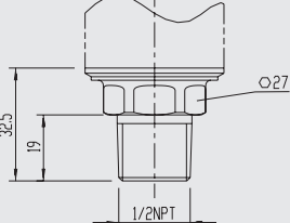
1/2 NPT ANSI/ASME B1.20.1 max. 1,000 bar
