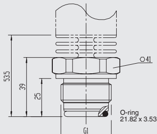
G 1 hygienic, flush up to 150 °C
