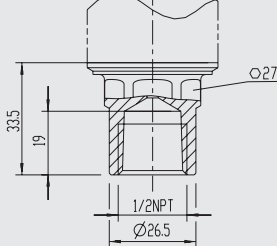
1/2 NPT female ANSI/ASME B1.20.1 max. 1,000 bar
