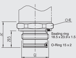
G 1 B, flush with O-ring
