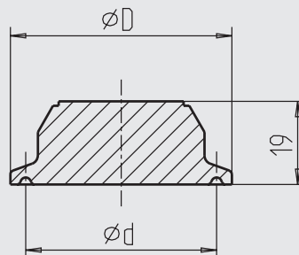
Clamp
