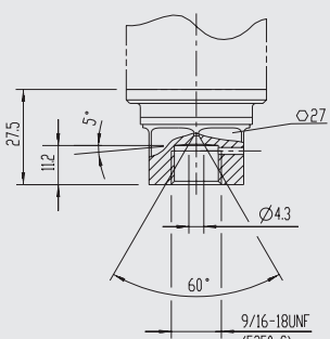
9/16-18 UNF female F 250-C from 1,600 bar
