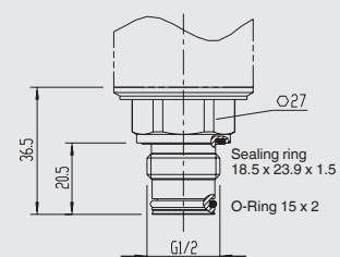
G 1/2 B, flush with O-ring
