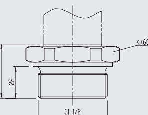
G 1 1/2 B, flush without O-ring
