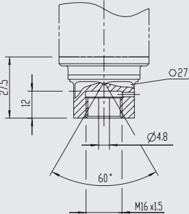
M16 x 1.5 female with sealing cone ab 1,600 bar
