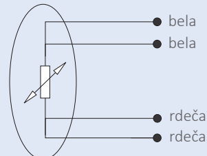
1 x Pt100, Pt1000... 4-vodno
