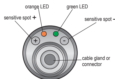
Top view of sensor control elements
